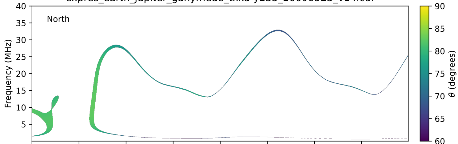
expres_earth_jupiter_ganymede_txka-y235_20090923_v14.cdf
