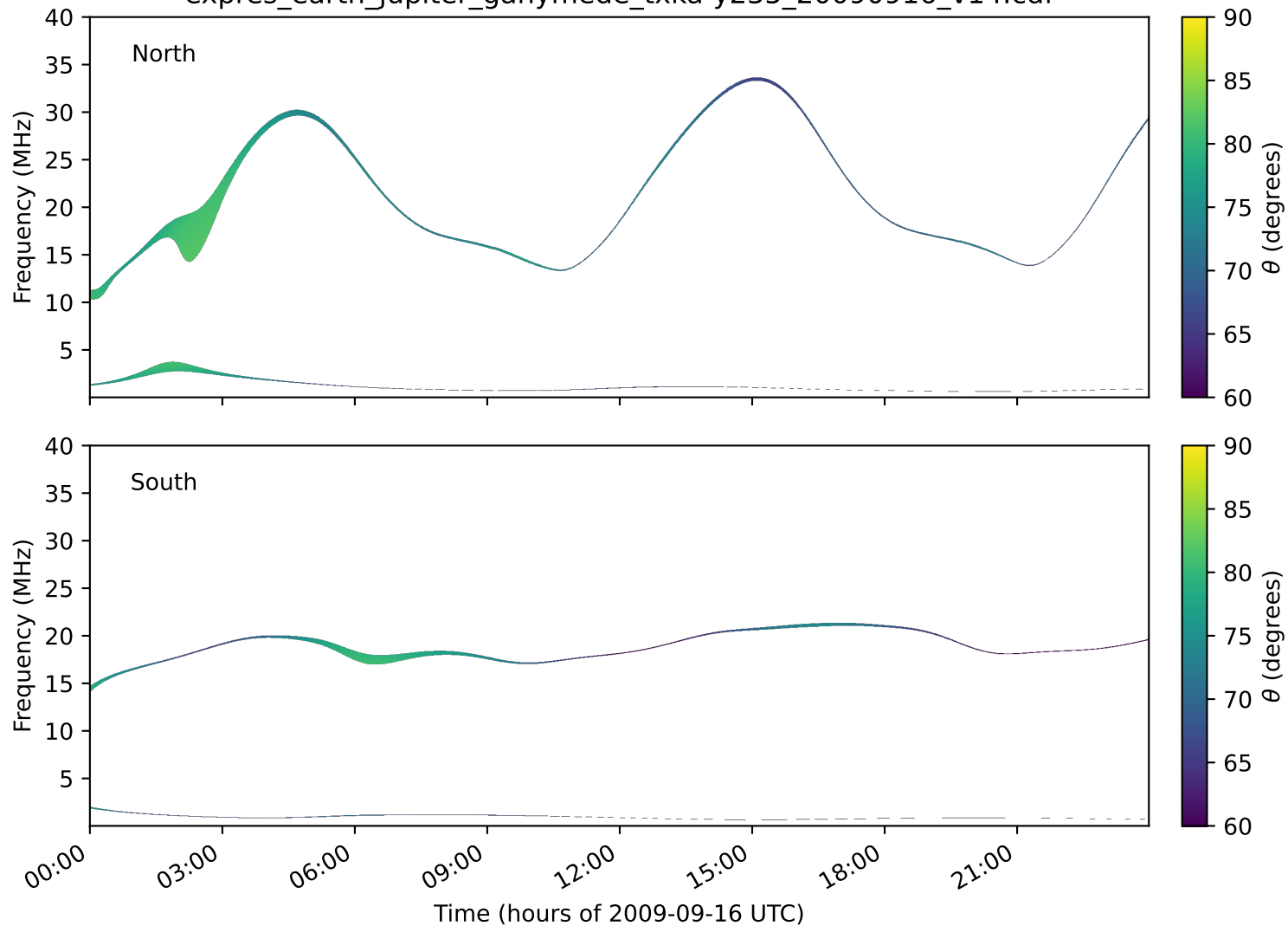
expres_earth_jupiter_ganymede_txka-y235_20090916_v14.cdf
