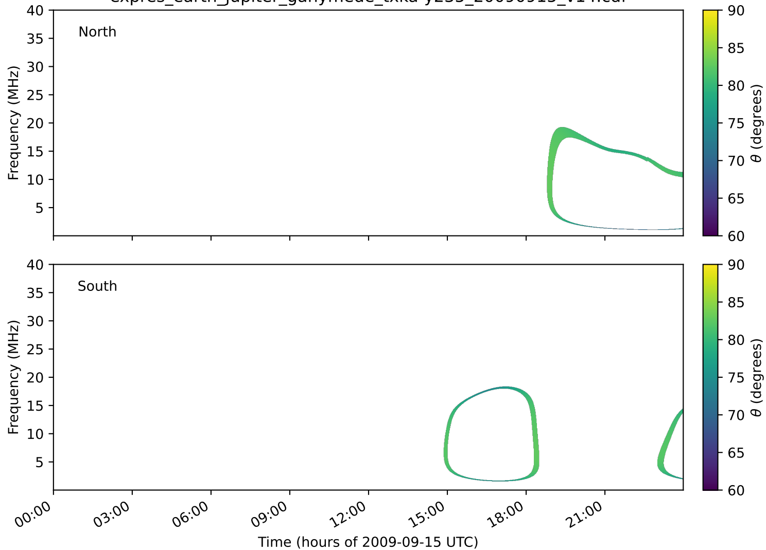
expres_earth_jupiter_ganymede_txka-y235_20090915_v14.cdf
