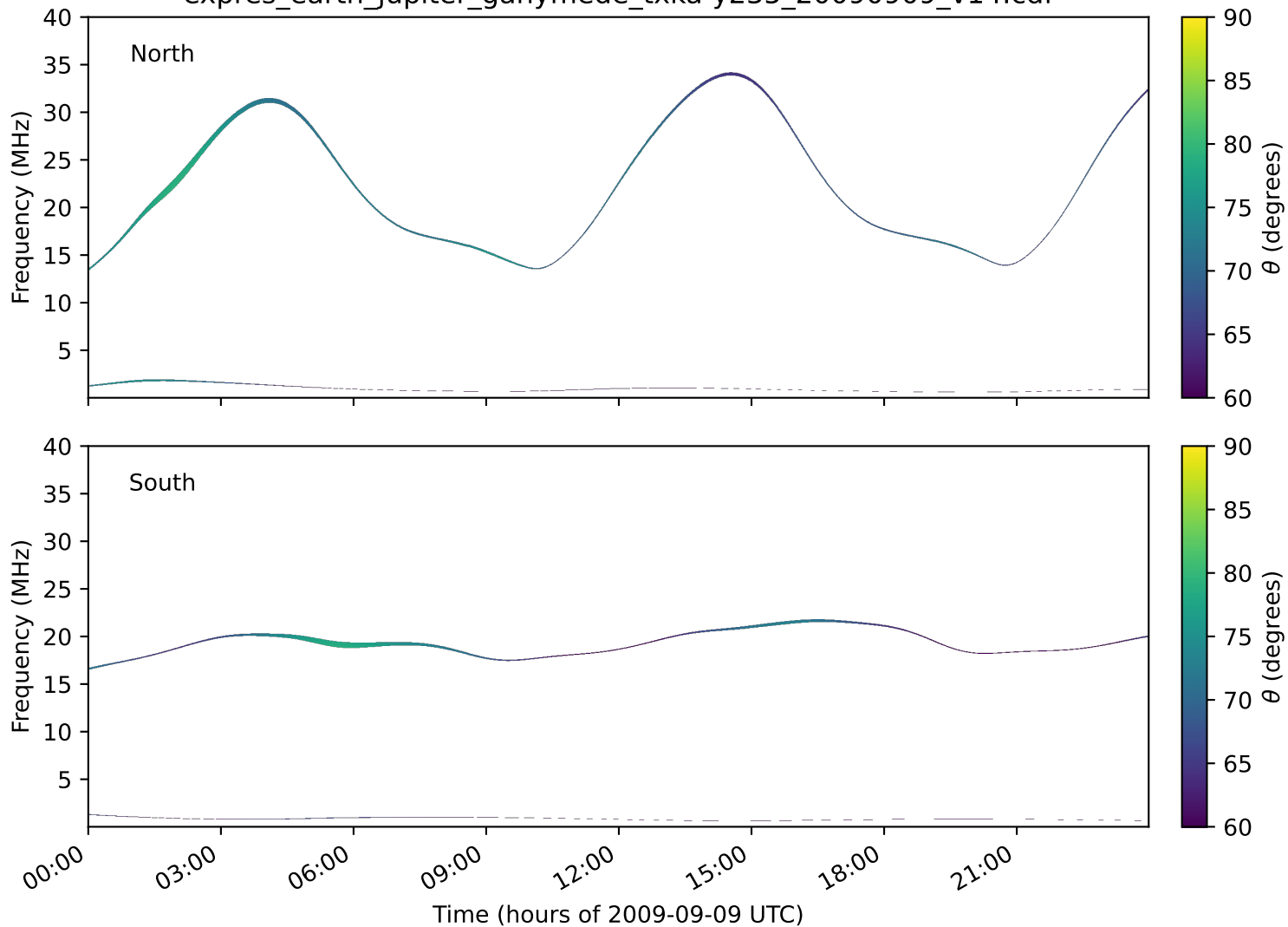
expres_earth_jupiter_ganymede_txka-y235_20090909_v14.cdf
