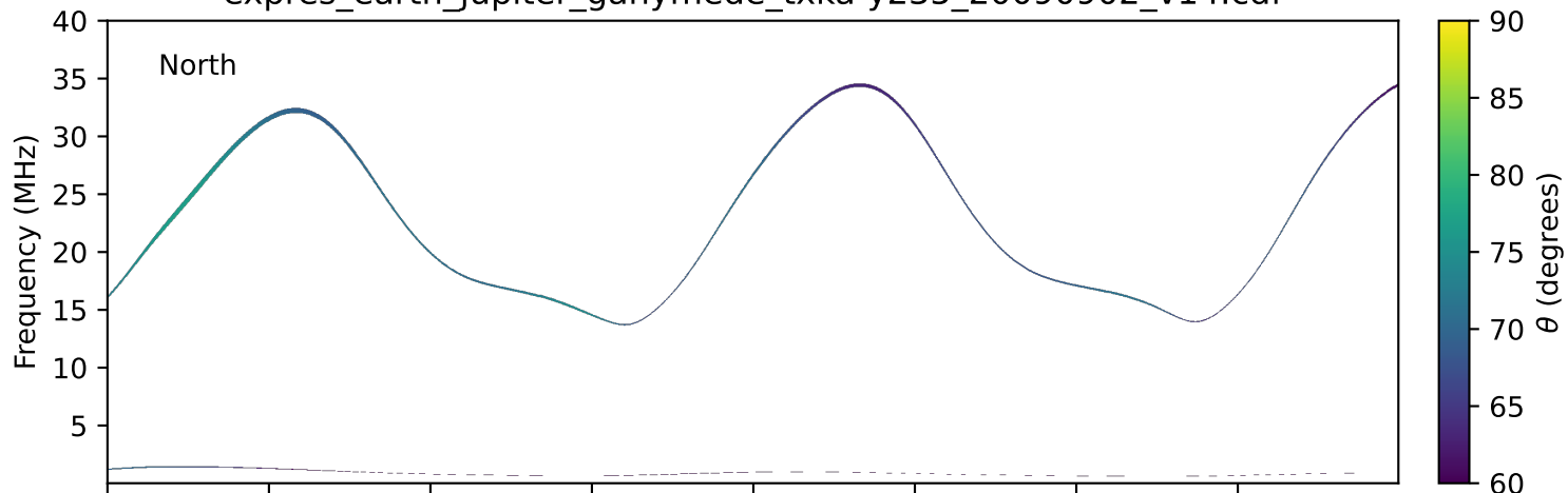
expres_earth_jupiter_ganymede_txka-y235_20090902_v14.cdf
