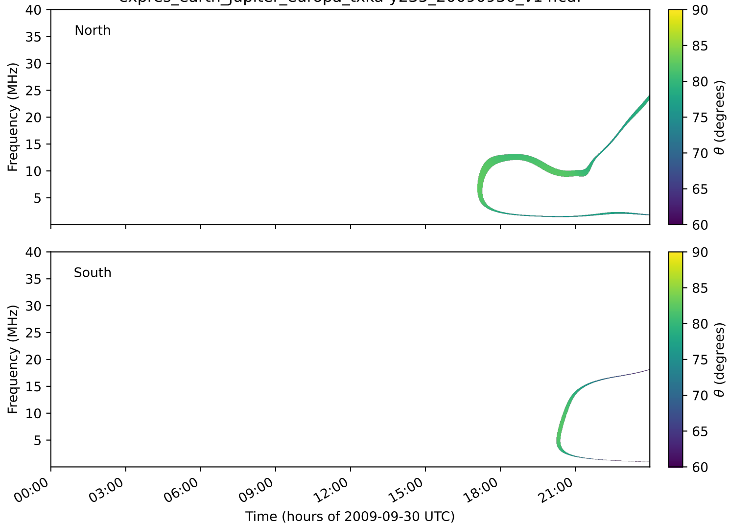
expres_earth_jupiter_europa_txka-y235_20090930_v14.cdf
