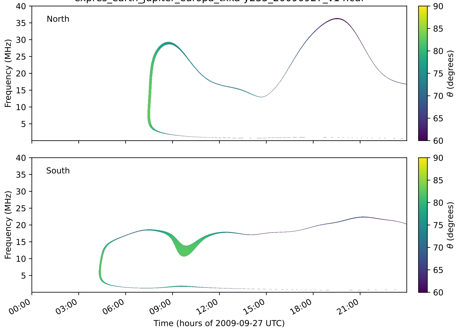
expres_earth_jupiter_europa_txka-y235_20090927_v14.cdf
