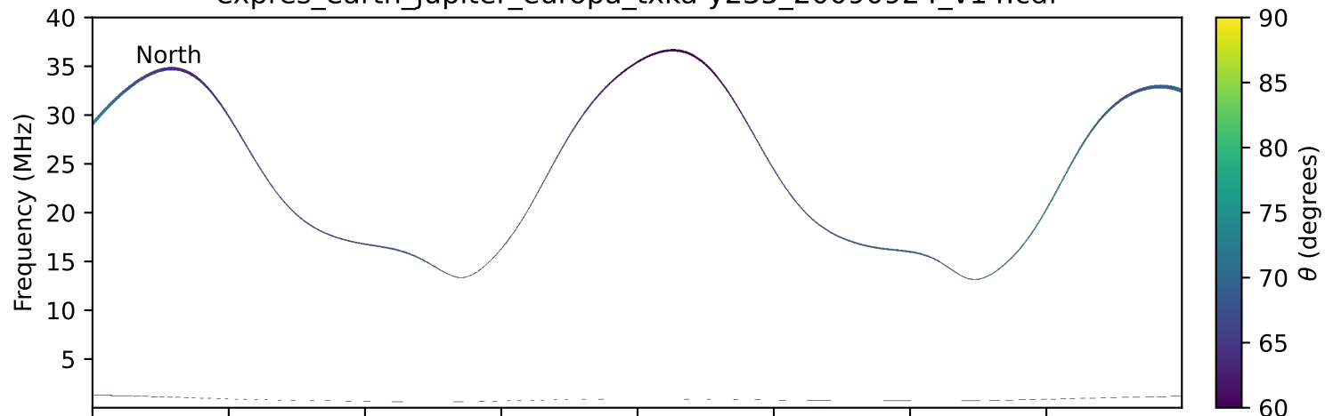
expres_earth_jupiter_europa_txka-y235_20090924_v14.cdf
