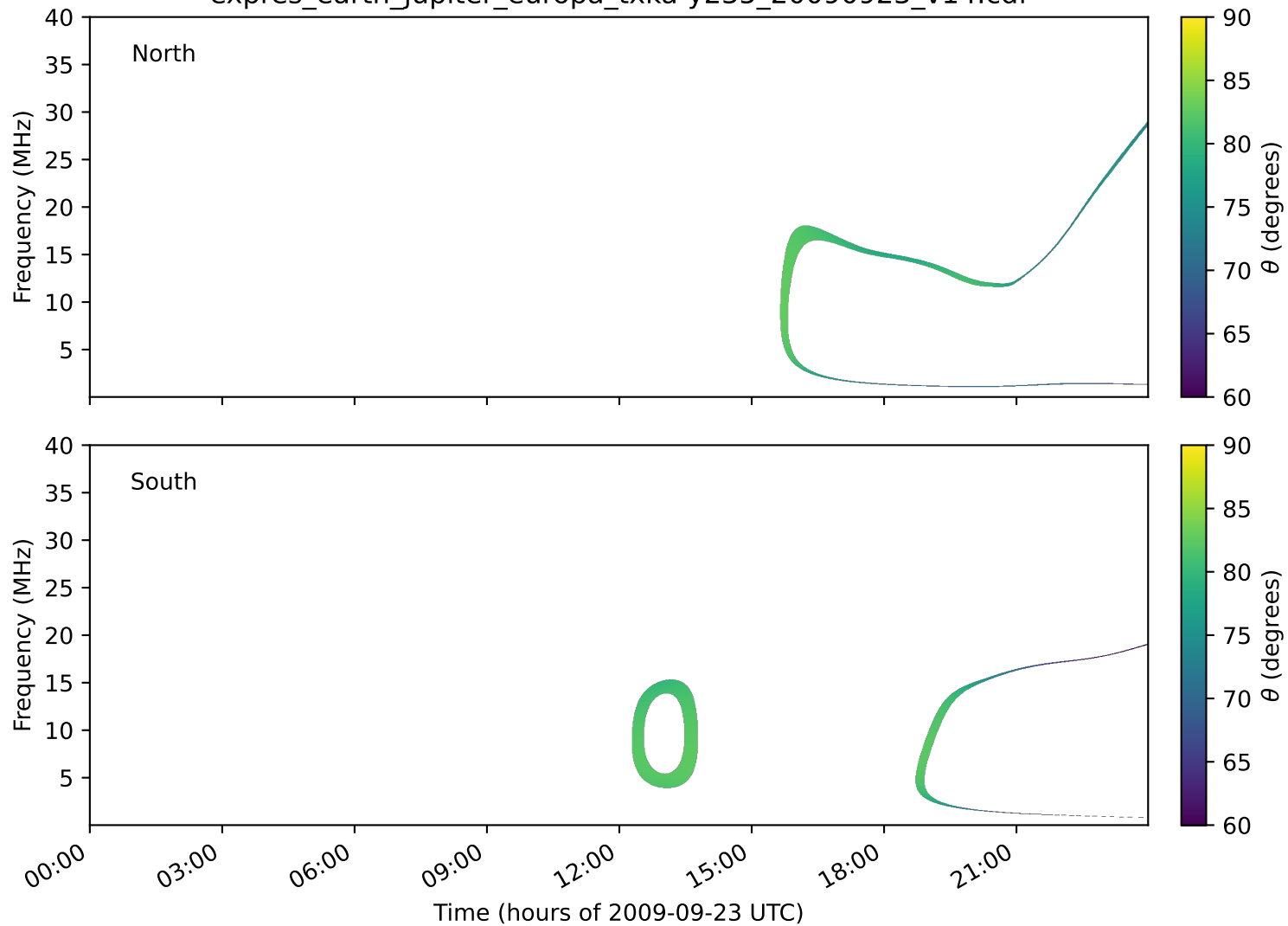
expres_earth_jupiter_europa_txka-y235_20090923_v14.cdf
