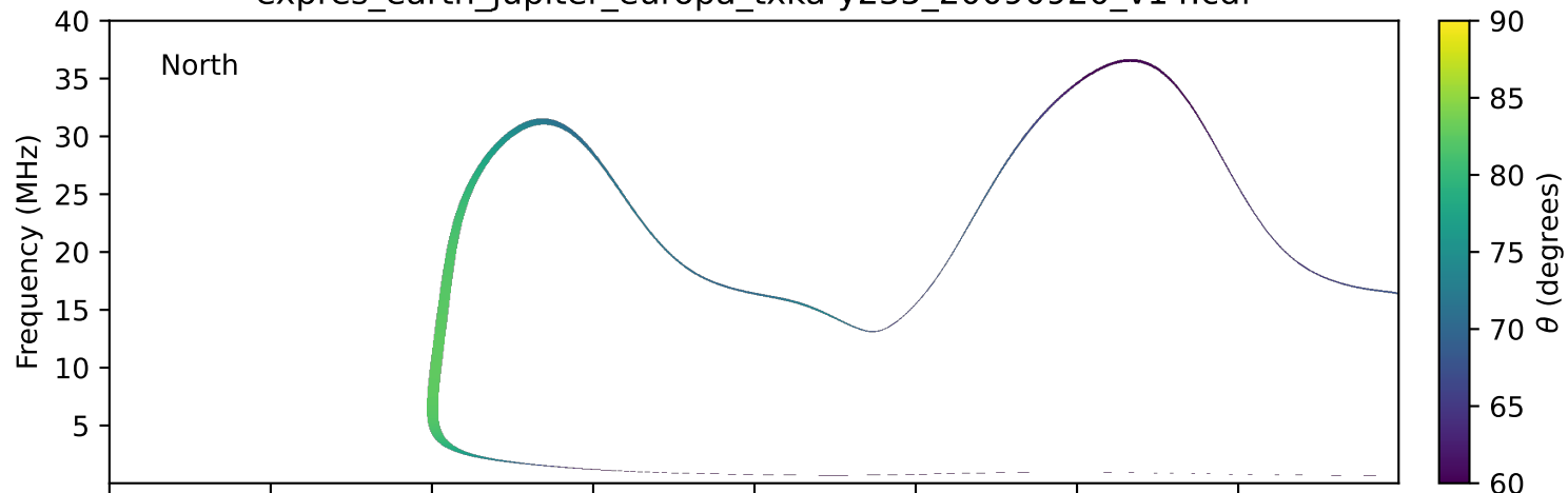
expres_earth_jupiter_europa_txka-y235_20090920_v14.cdf
