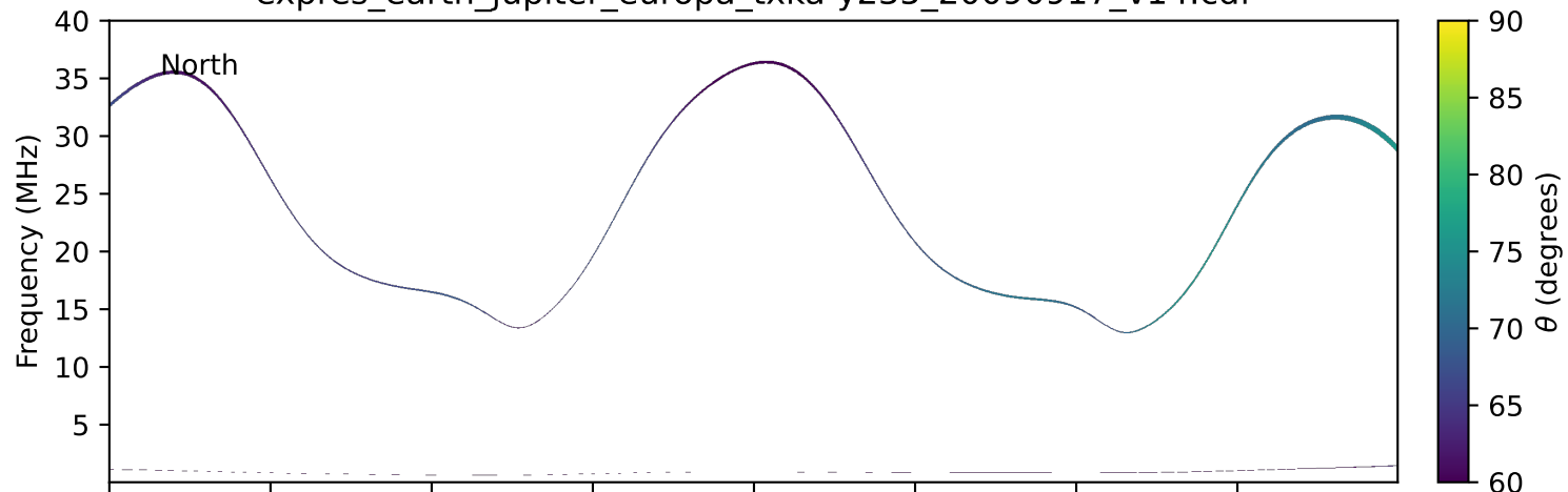
expres_earth_jupiter_europa_txka-y235_20090917_v14.cdf
