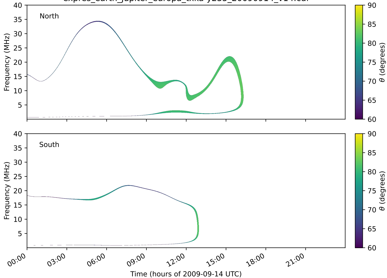
expres_earth_jupiter_europa_txka-y235_20090914_v14.cdf
