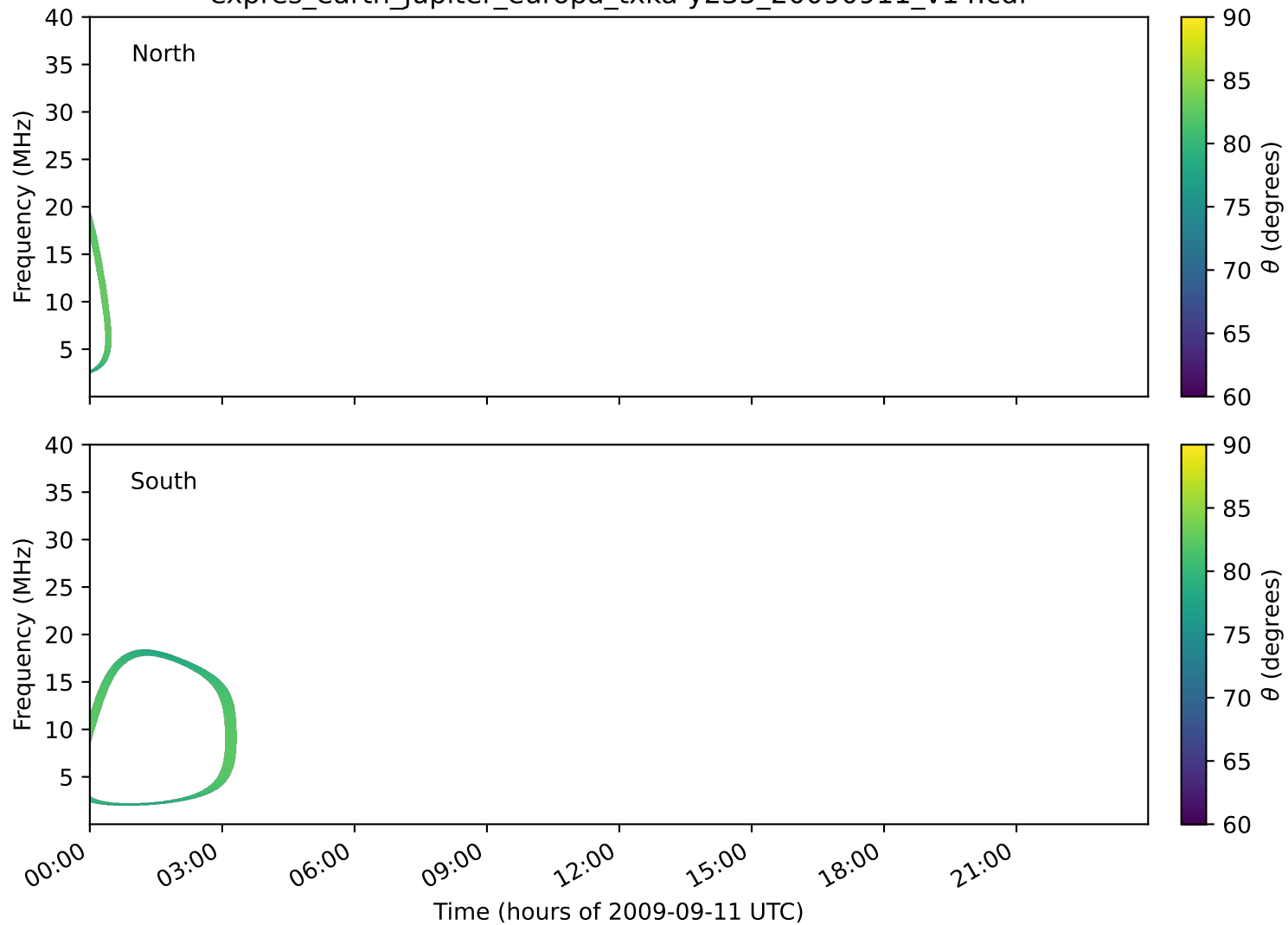
expres_earth_jupiter_europa_txka-y235_20090911_v14.cdf
