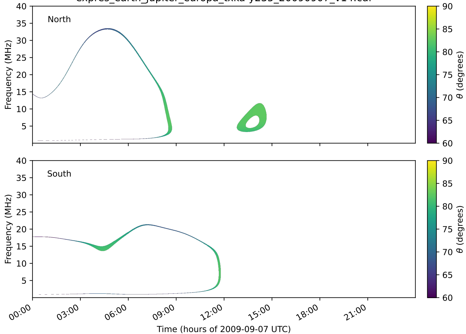
expres_earth_jupiter_europa_txka-y235_20090907_v14.cdf
