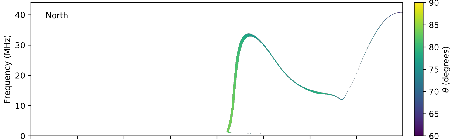
expres_earth_jupiter_europa_jrm09_lossc-wid1deg_3kev_20090909_v01.cdf
