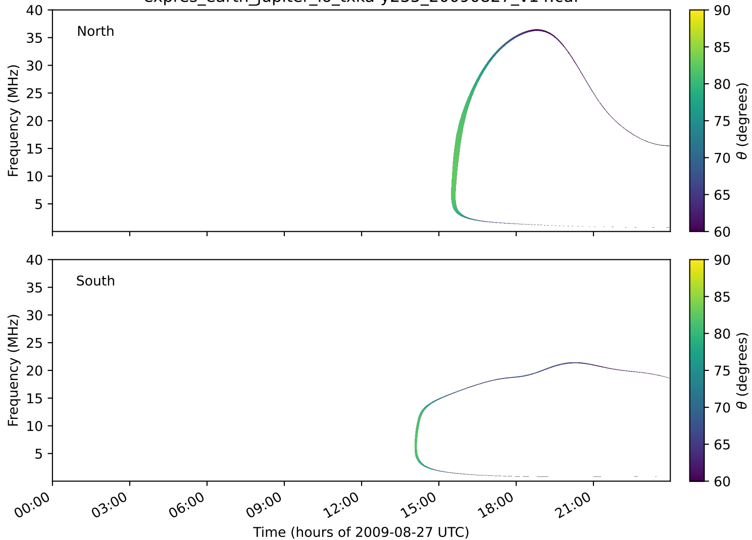
expres_earth_jupiter_io_txka-y235_20090827_v14.cdf
