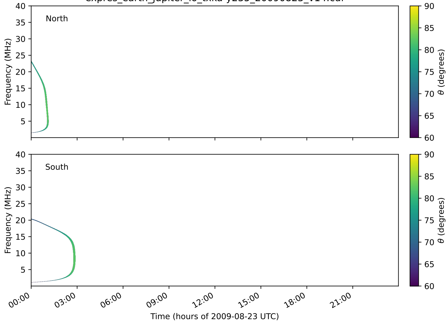
expres_earth_jupiter_io_txka-y235_20090823_v14.cdf
