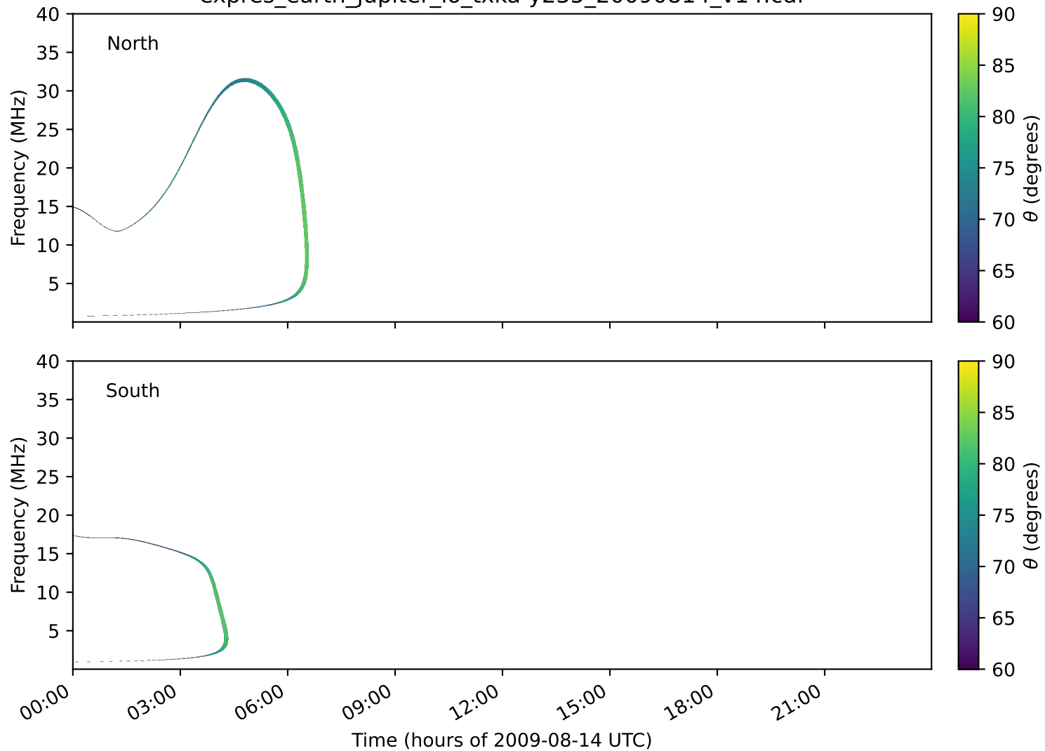
expres_earth_jupiter_io_txka-y235_20090814_v14.cdf
