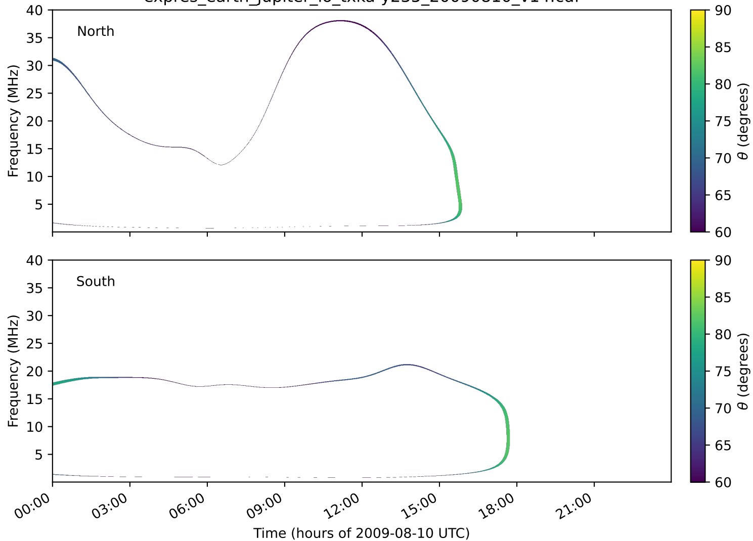
expres_earth_jupiter_io_txka-y235_20090810_v14.cdf
