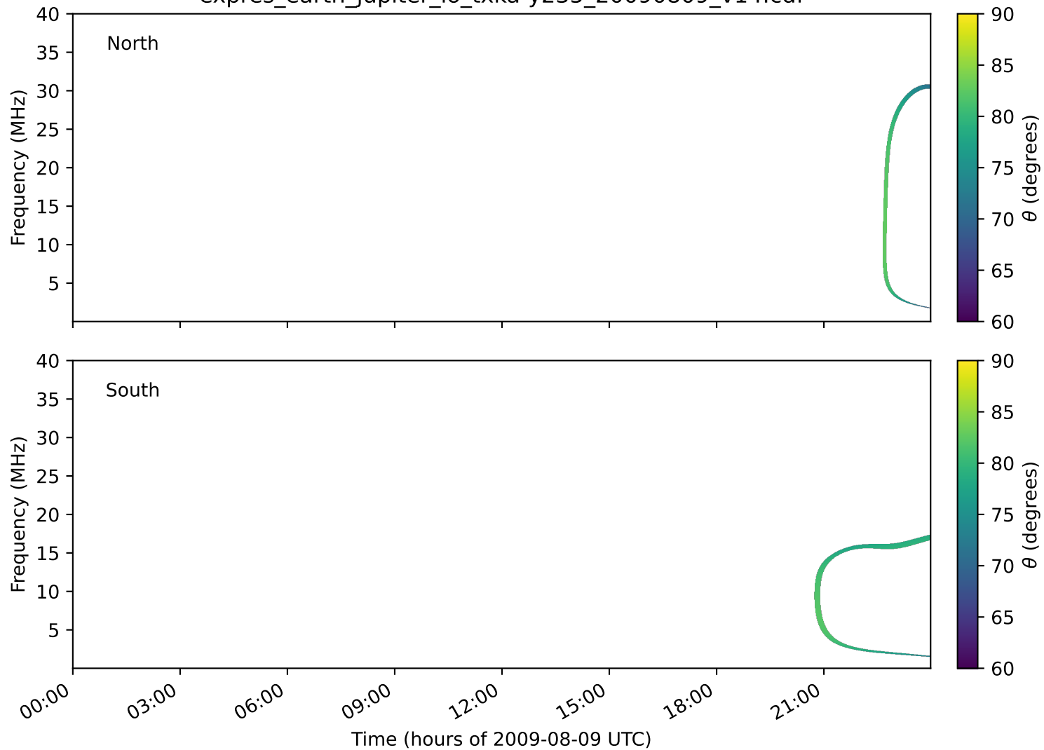
expres_earth_jupiter_io_txka-y235_20090809_v14.cdf
