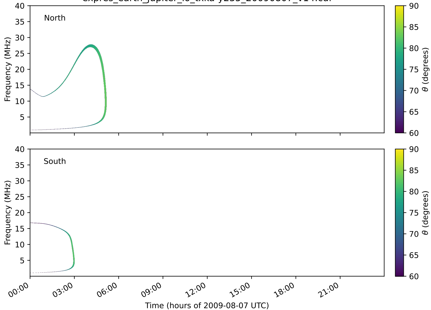
expres_earth_jupiter_io_txka-y235_20090807_v14.cdf
