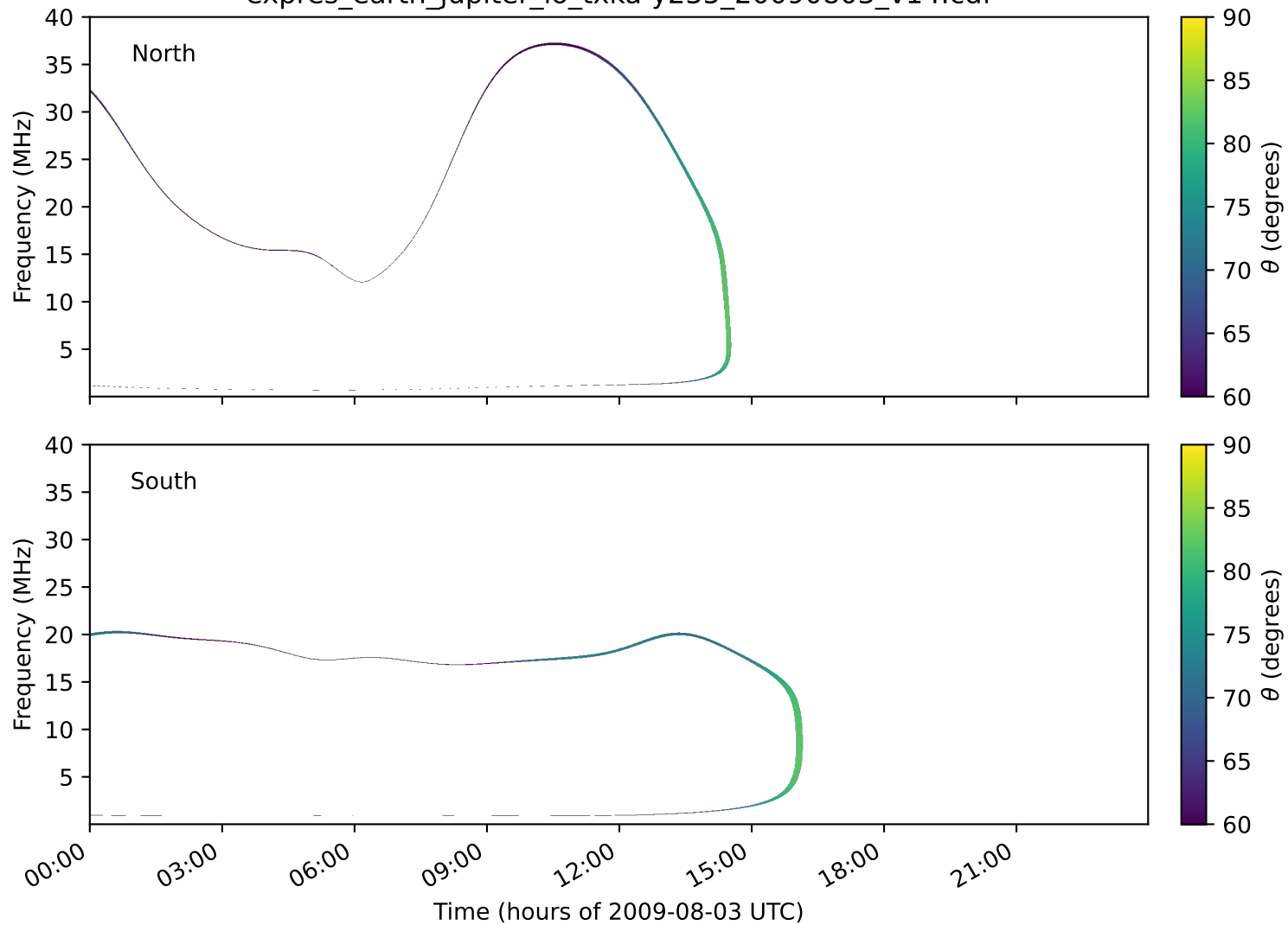
expres_earth_jupiter_io_txka-y235_20090803_v14.cdf
