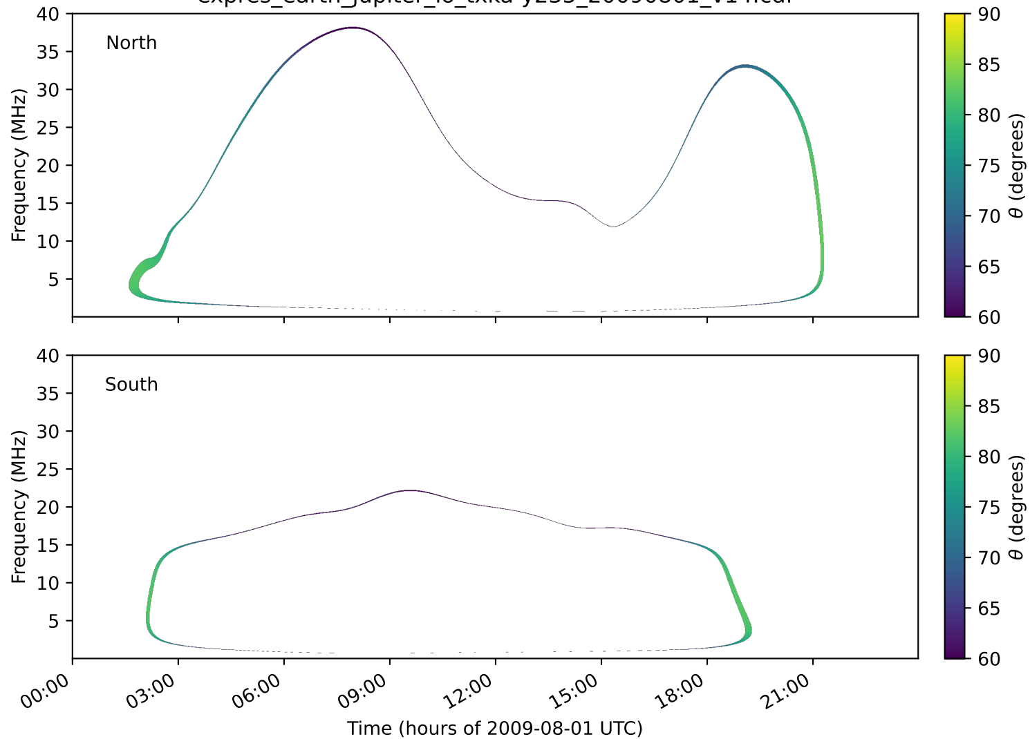
expres_earth_jupiter_io_txka-y235_20090801_v14.cdf
