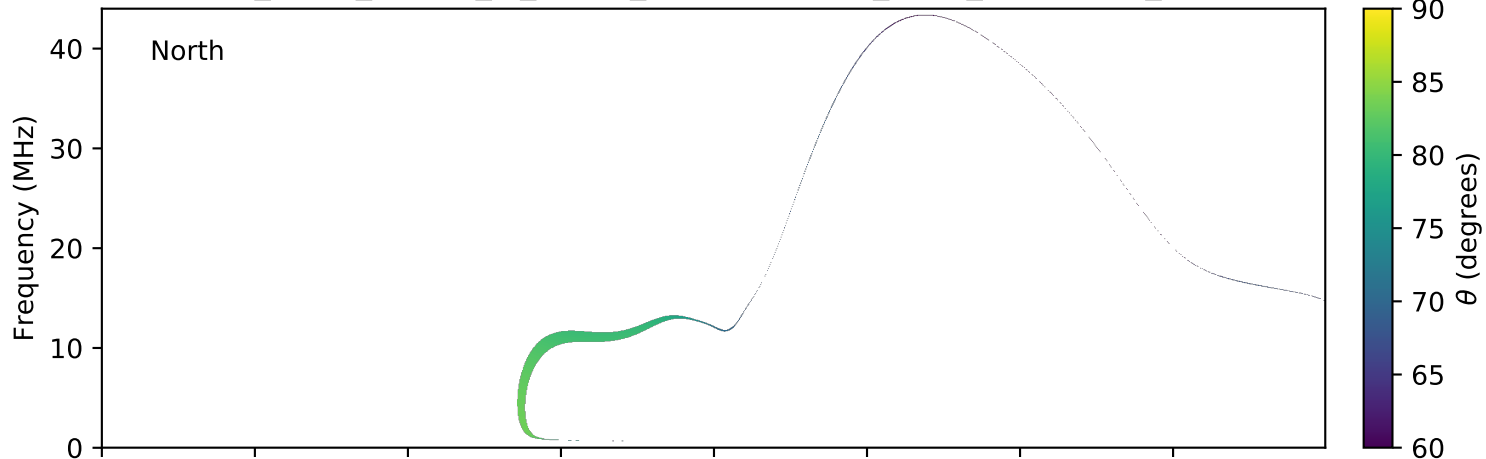
expres_earth_jupiter_io_jrm09_lossc-wid1deg_3kev_20090806_v01.cdf
