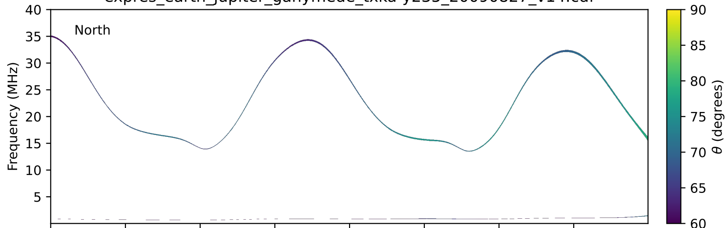
expres_earth_jupiter_ganymede_txka-y235_20090827_v14.cdf
