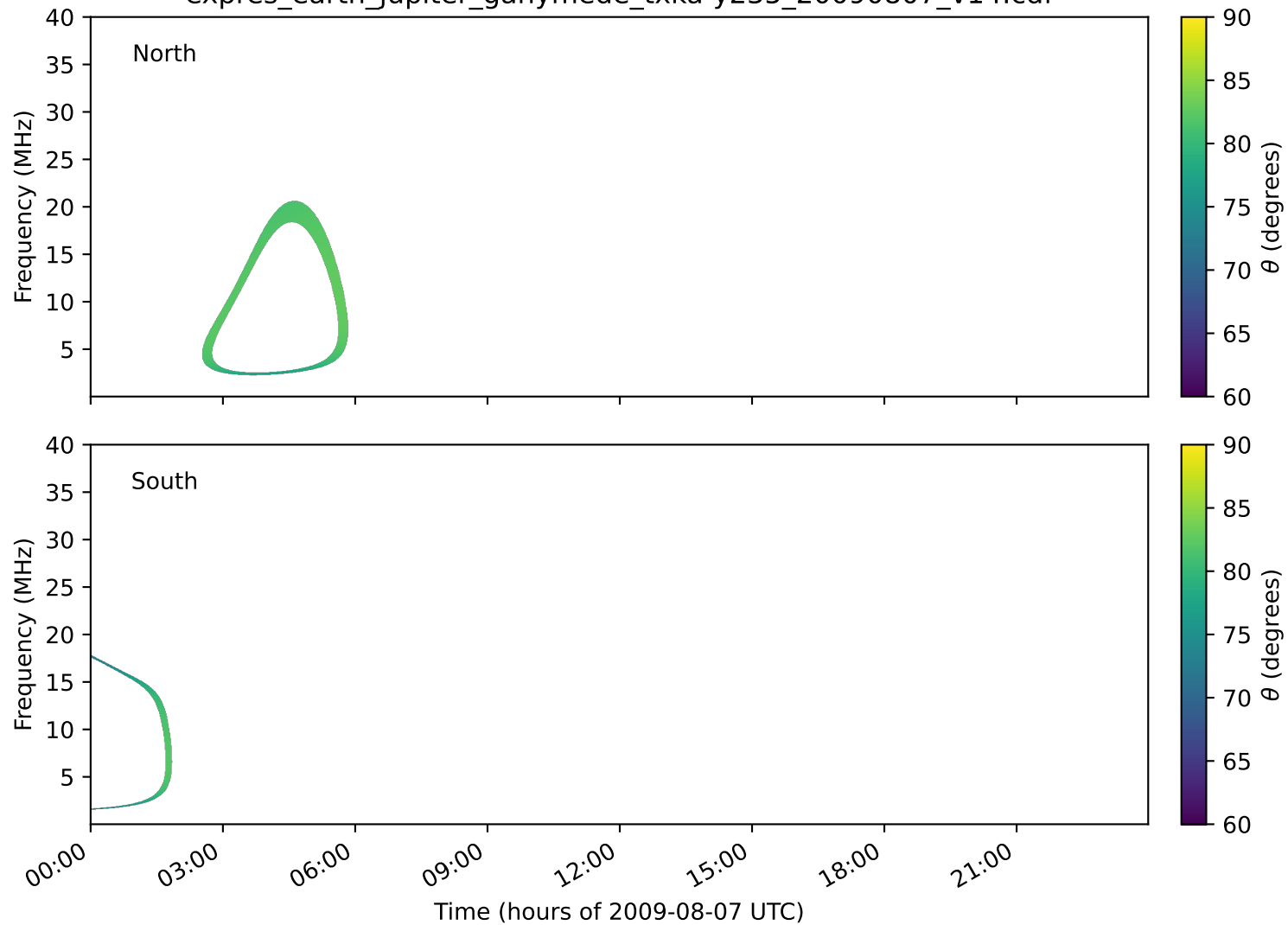
expres_earth_jupiter_ganymede_txka-y235_20090807_v14.cdf
