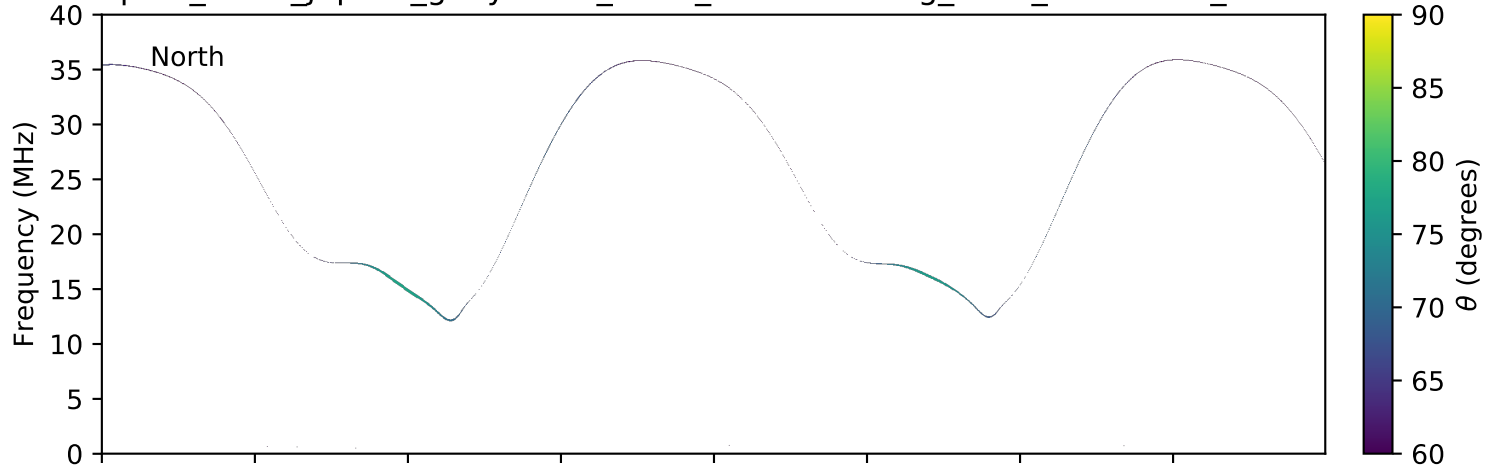
expres_earth_jupiter_ganymede_isaac_lossc-wid1deg_3kev_20090805_v01.cdf
