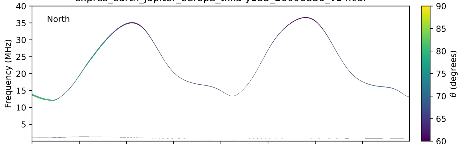
expres_earth_jupiter_europa_txka-y235_20090830_v14.cdf
