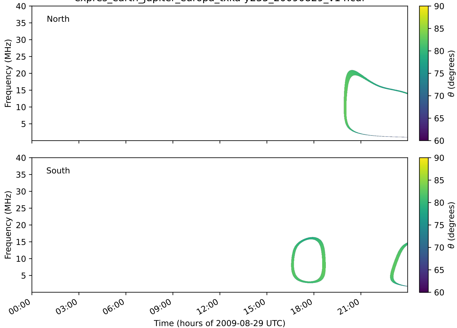
expres_earth_jupiter_europa_txka-y235_20090829_v14.cdf
