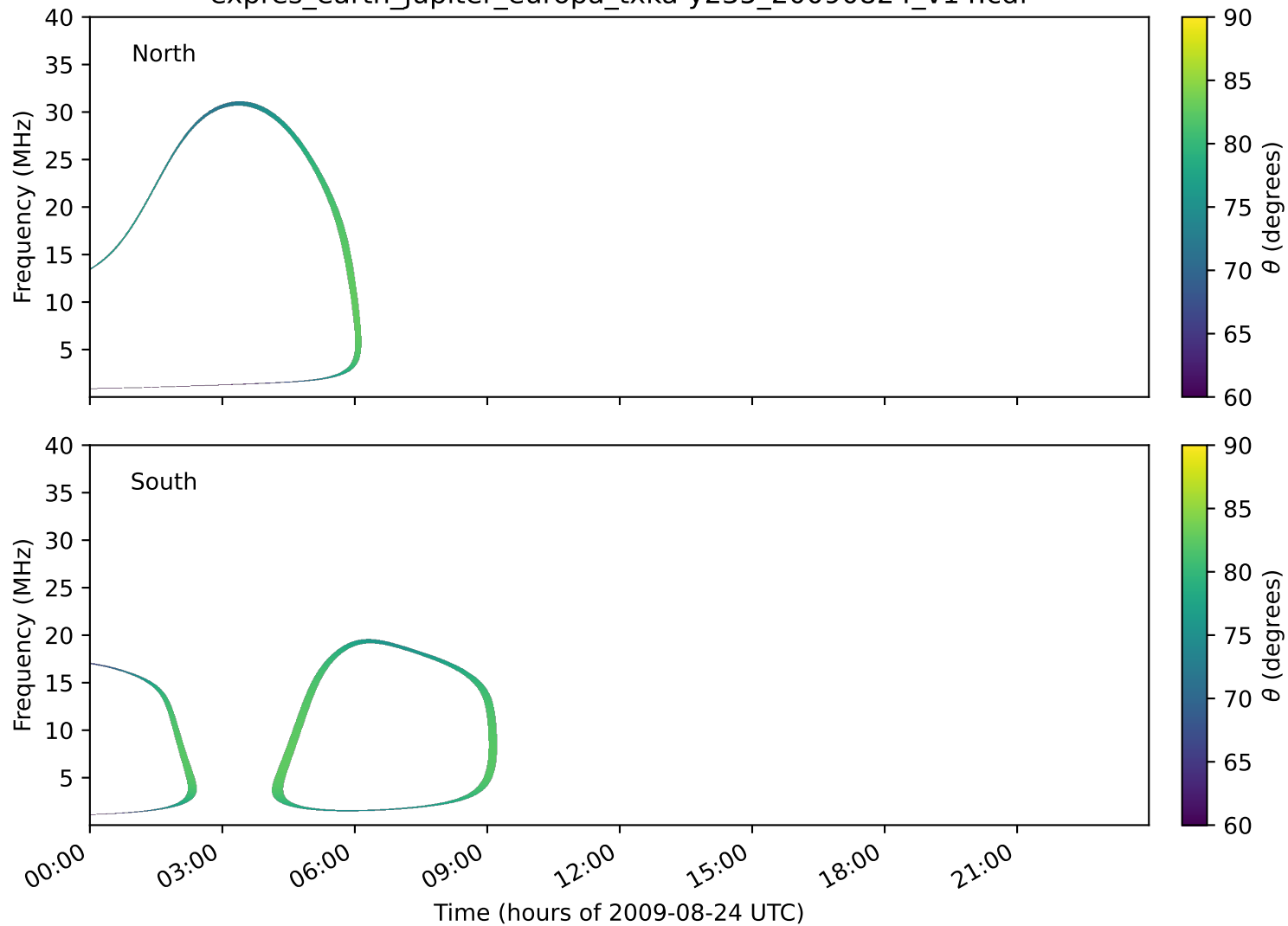
expres_earth_jupiter_europa_txka-y235_20090824_v14.cdf
