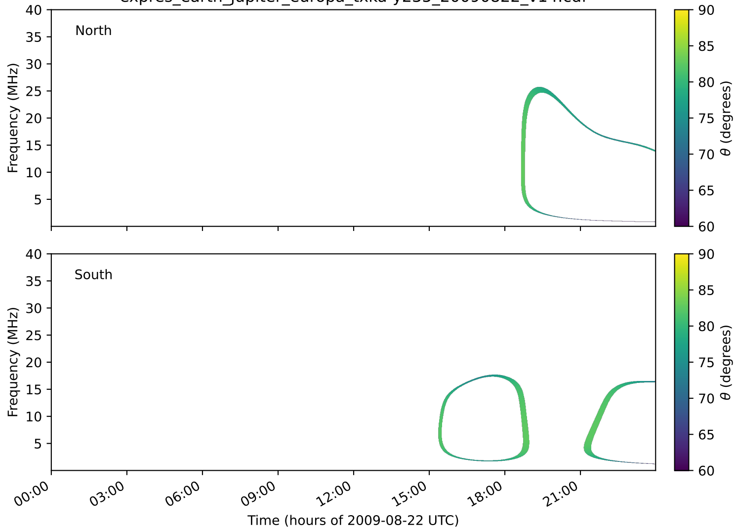
expres_earth_jupiter_europa_txka-y235_20090822_v14.cdf
