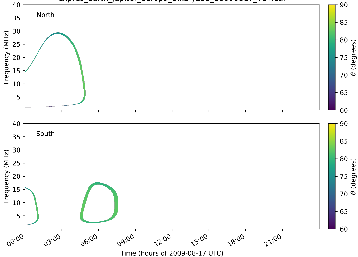
expres_earth_jupiter_europa_txka-y235_20090817_v14.cdf
