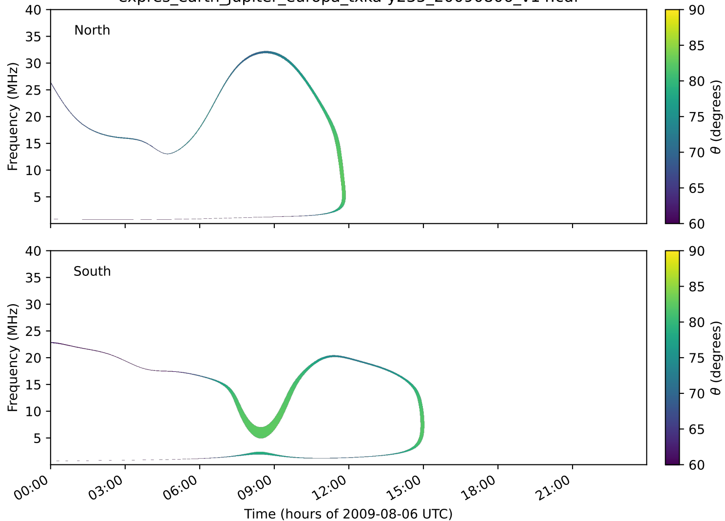
expres_earth_jupiter_europa_txka-y235_20090806_v14.cdf
