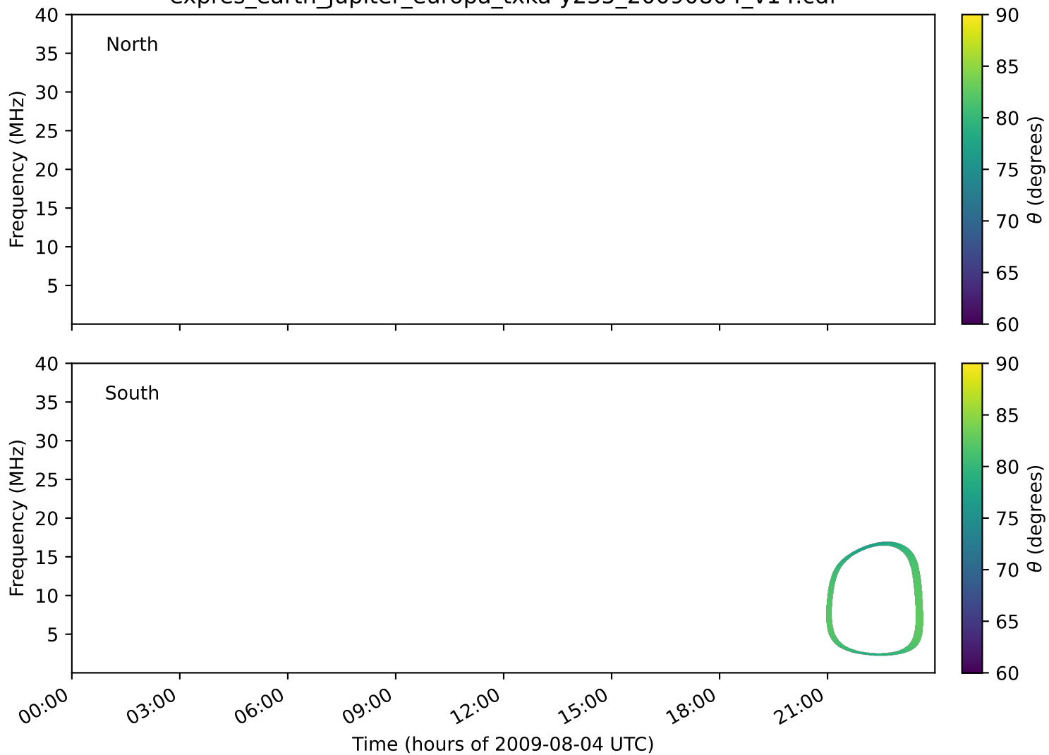
expres_earth_jupiter_europa_txka-y235_20090804_v14.cdf
