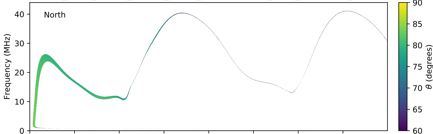
expres_earth_jupiter_europa_jrm09_lossc-wid1deg_3kev_20090805_v01.cdf
