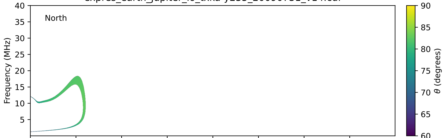
expres_earth_jupiter_io_txka-y235_20090731_v14.cdf
