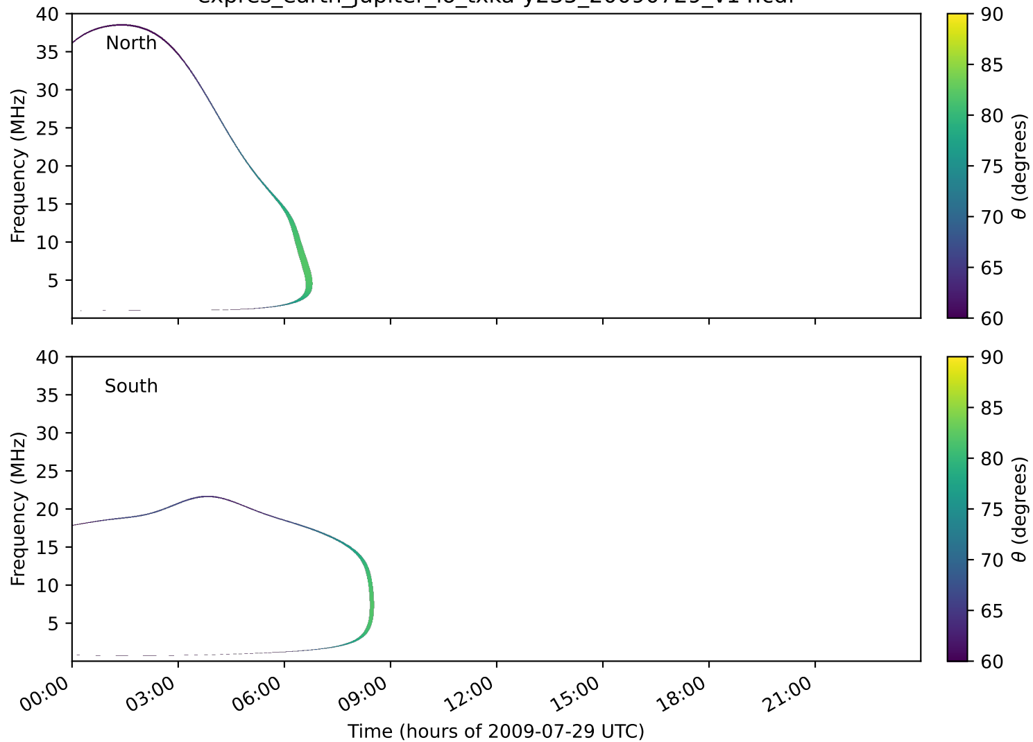
expres_earth_jupiter_io_txka-y235_20090729_v14.cdf
