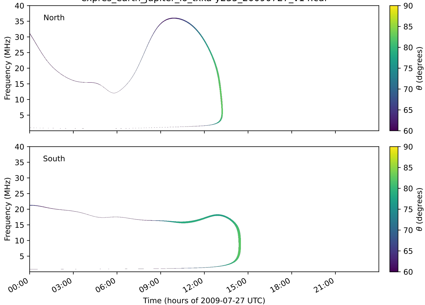
expres_earth_jupiter_io_txka-y235_20090727_v14.cdf
