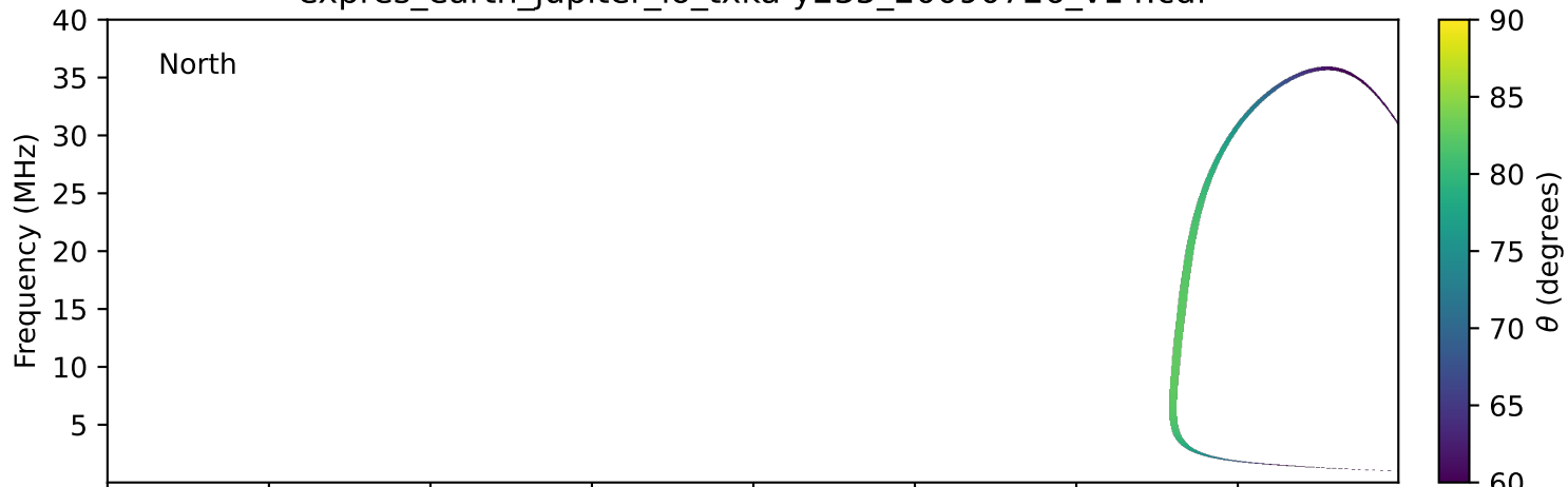
expres_earth_jupiter_io_txka-y235_20090726_v14.cdf
