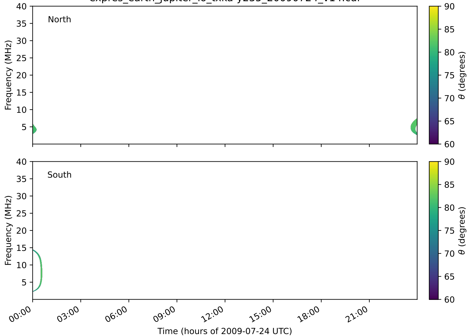
expres_earth_jupiter_io_txka-y235_20090724_v14.cdf
