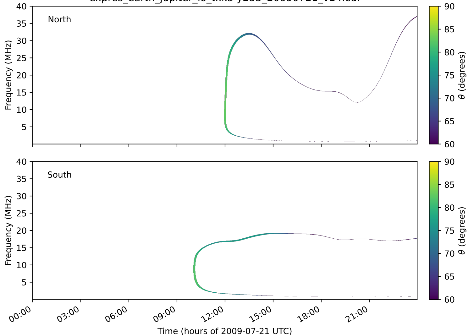
expres_earth_jupiter_io_txka-y235_20090721_v14.cdf
