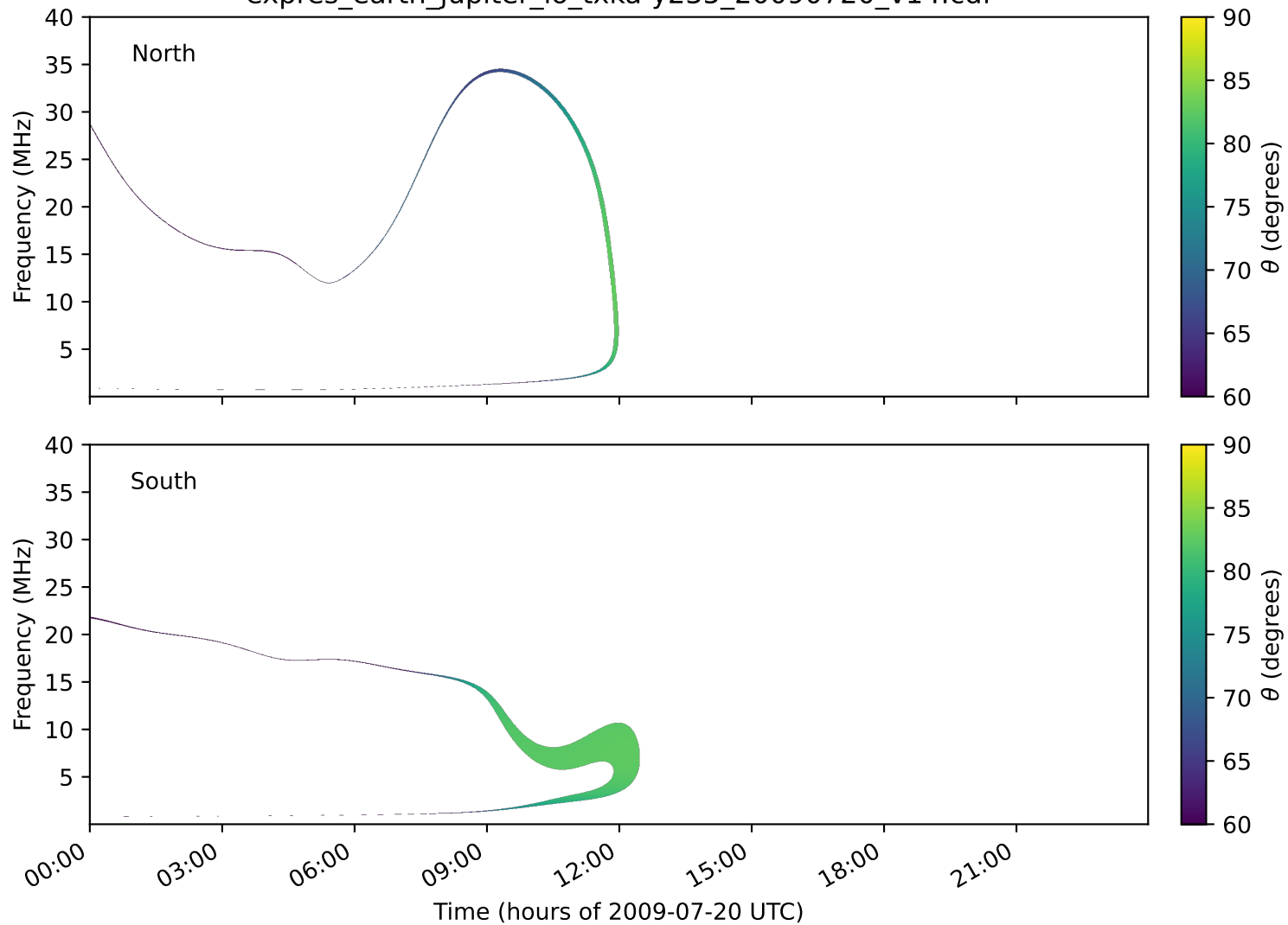
expres_earth_jupiter_io_txka-y235_20090720_v14.cdf
