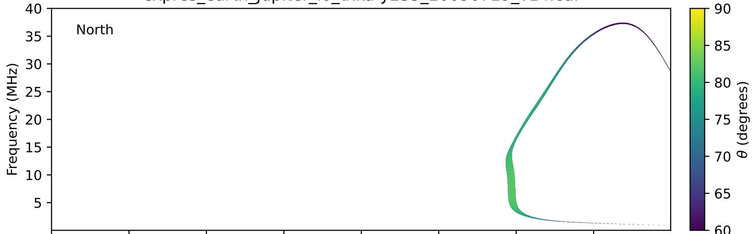
expres_earth_jupiter_io_txka-y235_20090719_v14.cdf
