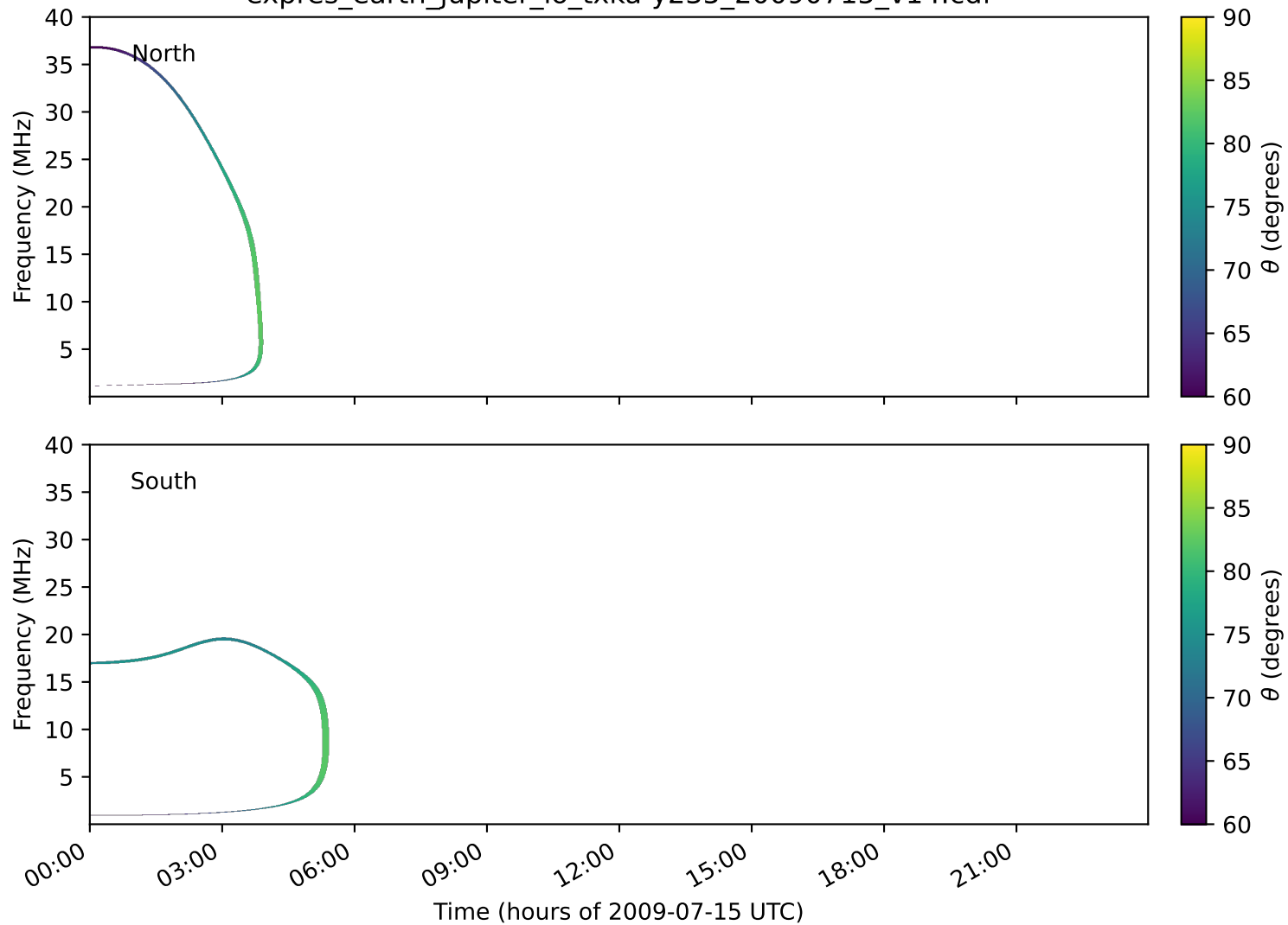
expres_earth_jupiter_io_txka-y235_20090715_v14.cdf
