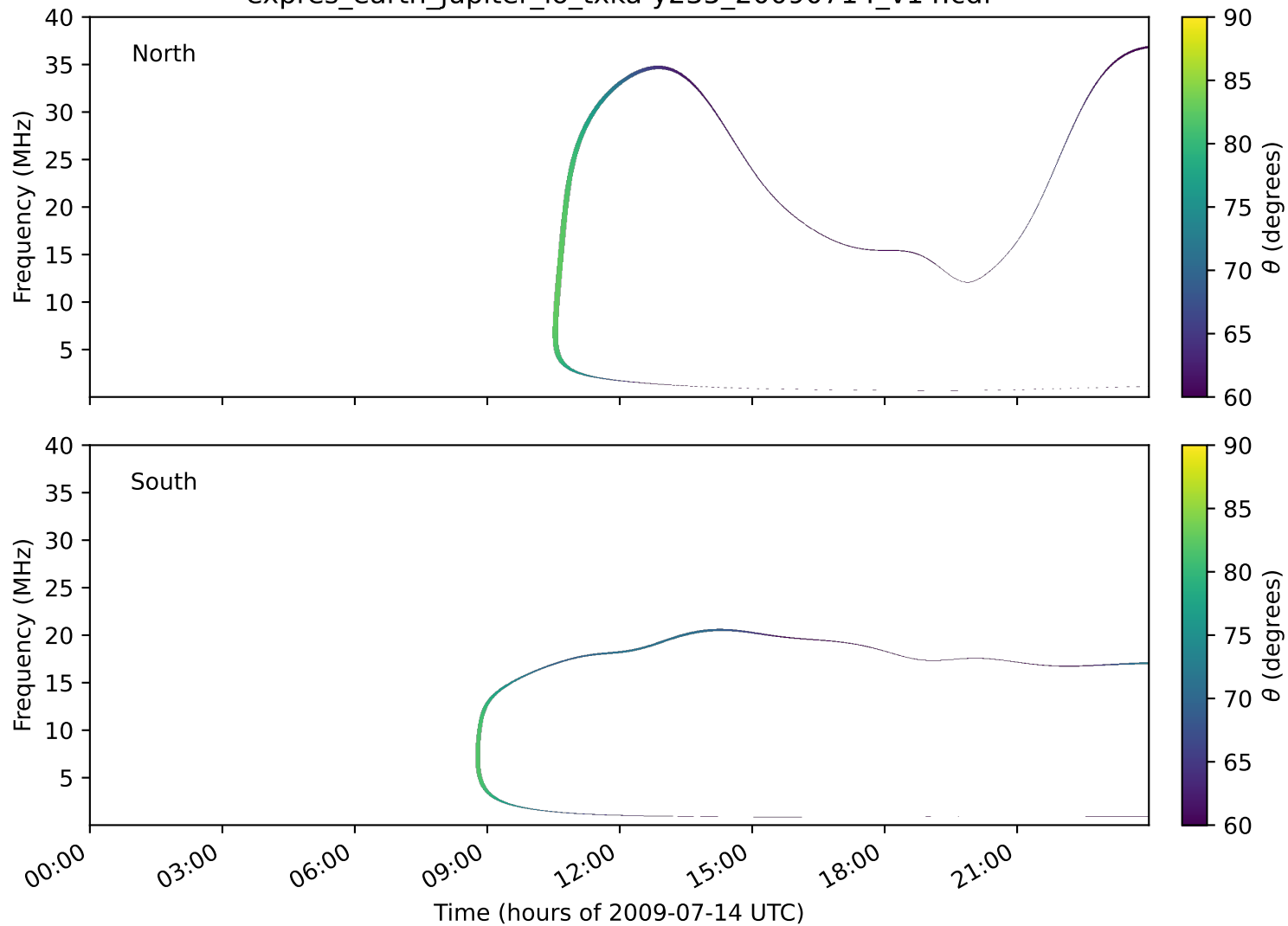
expres_earth_jupiter_io_txka-y235_20090714_v14.cdf
