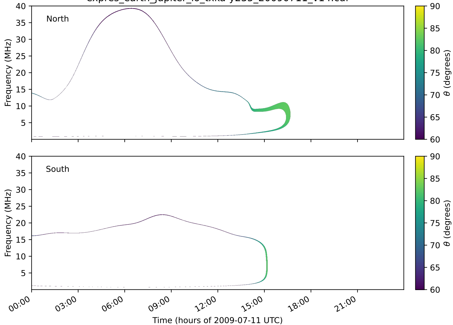
expres_earth_jupiter_io_txka-y235_20090711_v14.cdf
