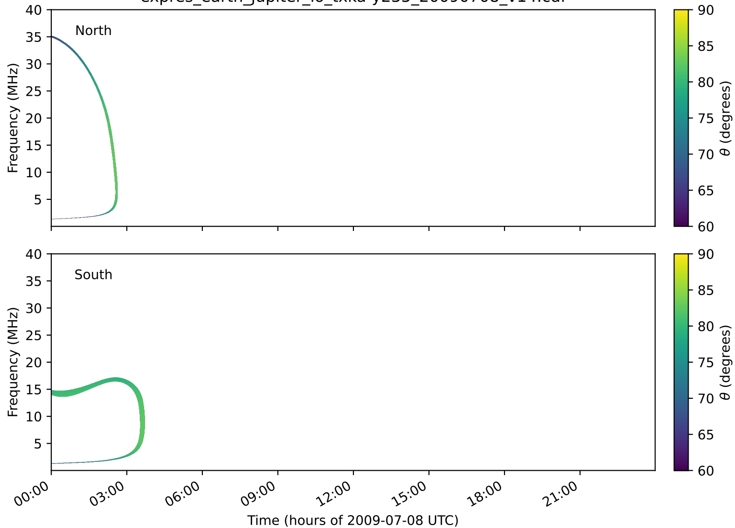
expres_earth_jupiter_io_txka-y235_20090708_v14.cdf
