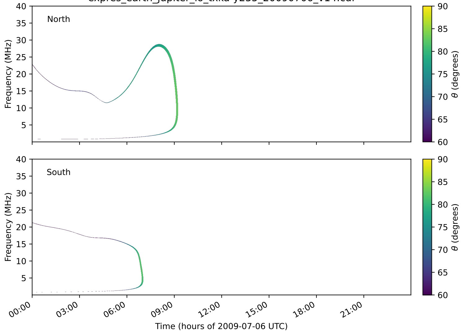
expres_earth_jupiter_io_txka-y235_20090706_v14.cdf
