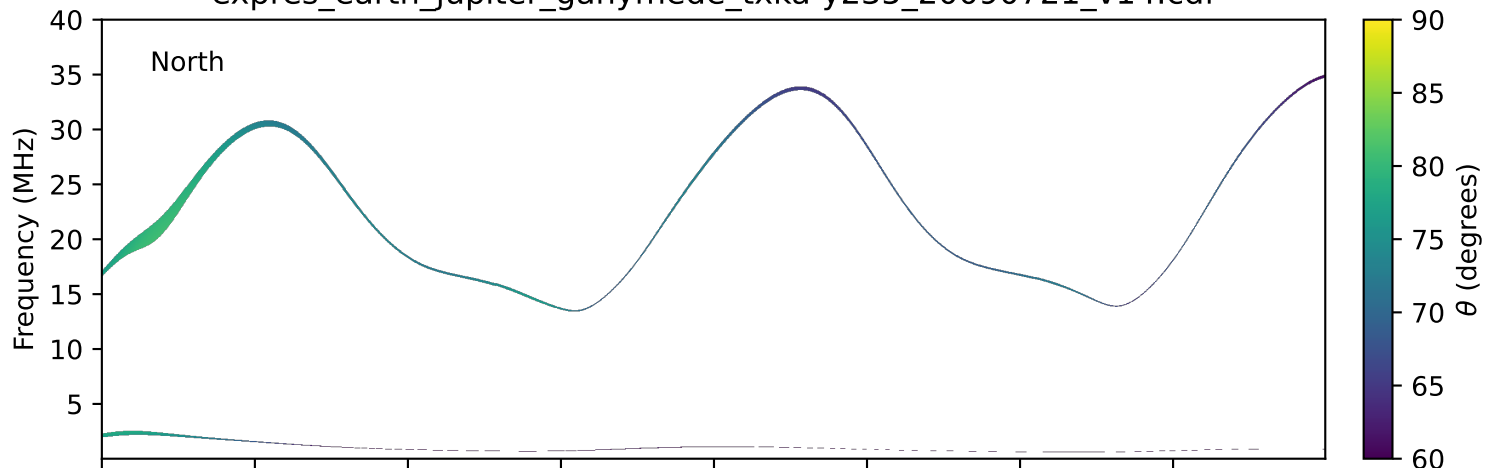
expres_earth_jupiter_ganymede_txka-y235_20090721_v14.cdf
