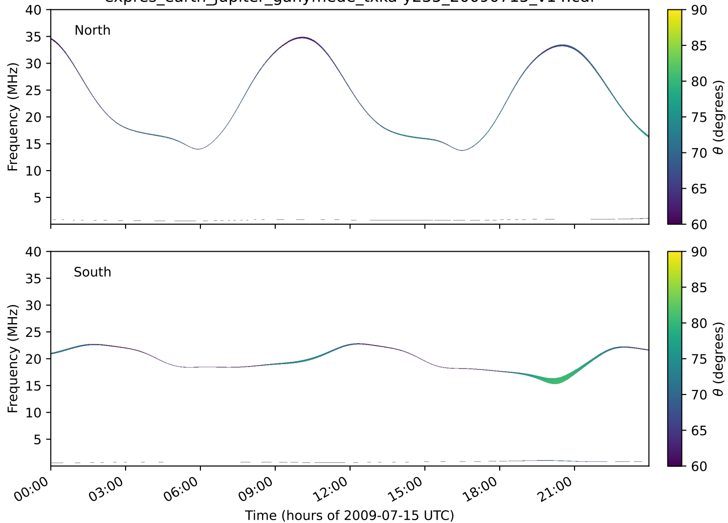
expres_earth_jupiter_ganymede_txka-y235_20090715_v14.cdf
